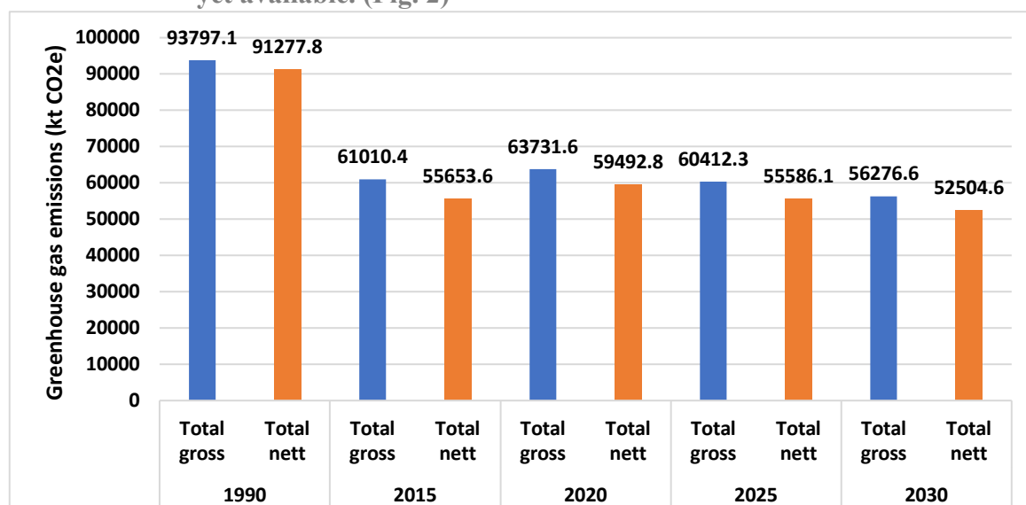
Fig2: Greenhouse gas emissions through complementary policies and measures 1990-2030 41 .
